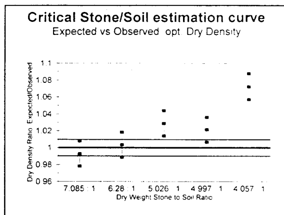
Figure 6. Graphic estimation of a likely critical ratio for limestone mixes. A ratio above one would indicate the critical stone to soil ratio had been crossed and compaction of the interstitial soil had likely experienced compaction. Error bars represent the range of ratio values due to the assigned acceptable error of each of the measurements ( \text{kg/m}^3 )
