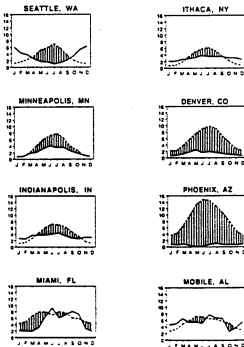
Figure 1. Climatic graphs of mean monthly precipitation and evaporation rates for eight major U.S. cities. The Y axis is in inches of precipitation and evaporation, the X axis is in months.
