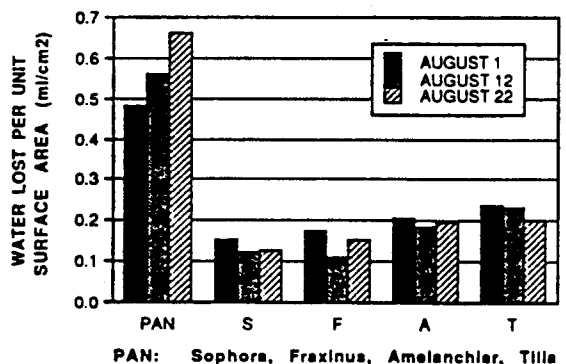
Figure 2. Evaporation from the pan compared with transpiration from the four tree species for a sampling of dates.
