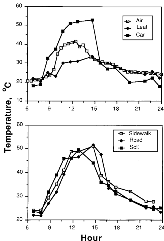
Figure 5. Diurnal temperature fluctuations for leaves and selected environmental surfaces on Columbus Avenue, August 16, 1983.
