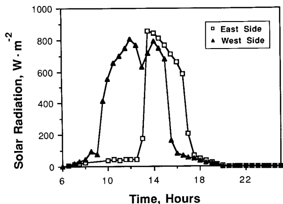
Figure 4. Diurnal pattern for solar radiation received by the eastern and western exposures of Columbus Avenue during late summer.
