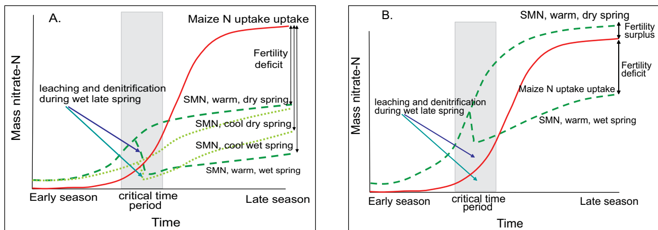
Figure 3. Conceptual gains and losses of soil mineral N and crop N over a growing season for a low soil N system (a), and a high soil N system (e.g., livestock; b). Broken and dotted lines represent SMN accumulations; solid line depicts maize N uptake.
