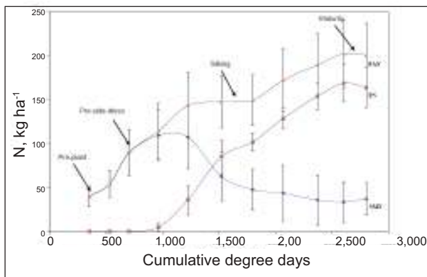
Figure 1. Accumulation of soil mineral N (SMN), total shoot N (PN), and plant available N (PAN) in the ON plots over the growing season. Bars describe standard deviations among years (from Kay et al., 2006; reprinted with permission).
