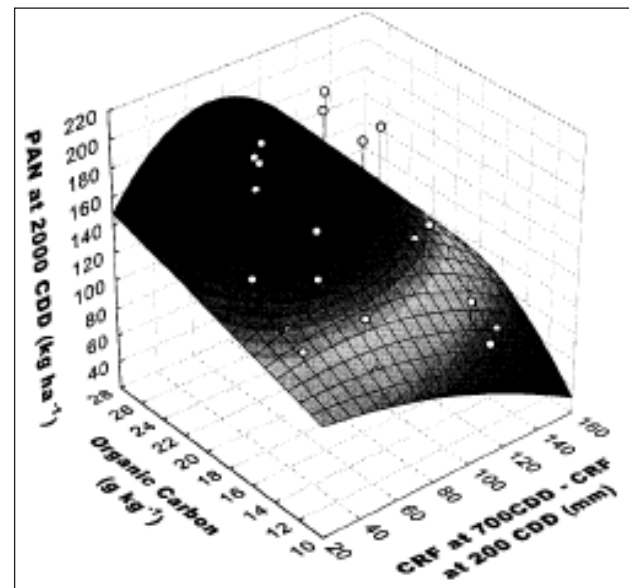
Figure 2. Variation in plant available N at 2000 CDD with organic carbon content and cumulative rainfall in the period 200 to 700 CDD for the barley-NT treatment, based on a regression equation with r^2=0.63 (from Kay et al., 2006; reprinted with permission).
